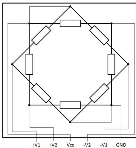
Figure 1: Circuit Diagram
